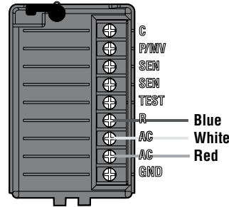
Smart Port Wiring Harness
